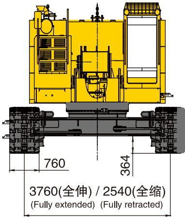
A向 ( 拆去主起重臂、人字架、变幅滑轮组等 ) A direction (main lifting boom, A-frame and luffing pulley block are removed away)
