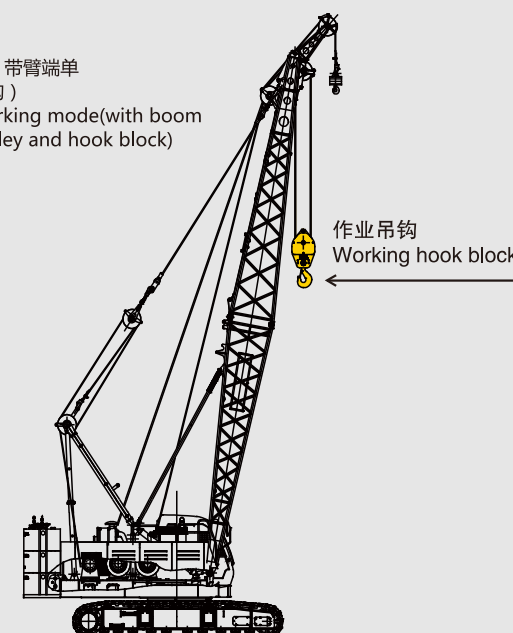
臂端单滑轮工况 (主臂带吊钩) Boom single pulley mode (with hook block)
